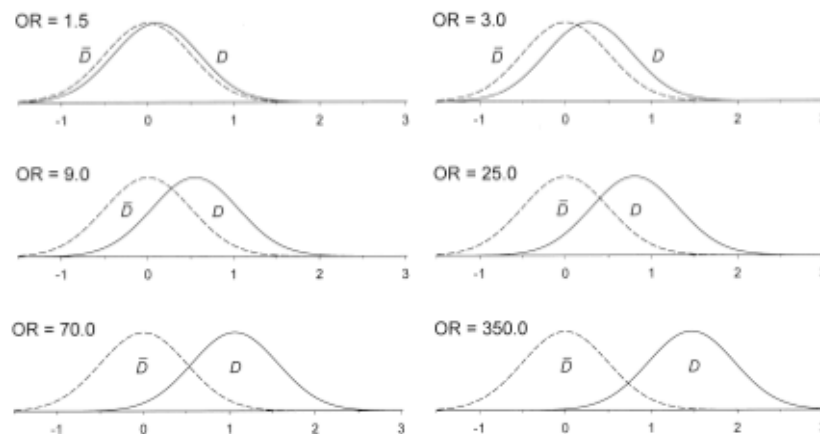
FIGURE 2. Probability distributions of a marker, X , in cases (solid curves) and controls (dashed curves) consistent with the logistic model \logit(P(D=1|X)) = \alpha + \beta X . It has been assumed that X has a mean of 0 and a standard deviation of 0.5 in controls so that a unit increase represents the difference between the 84th and 16th percentiles of X in controls. The marker is normally distributed, with the same variance in cases. The odds ratio (OR) per unit increase in X is shown.
