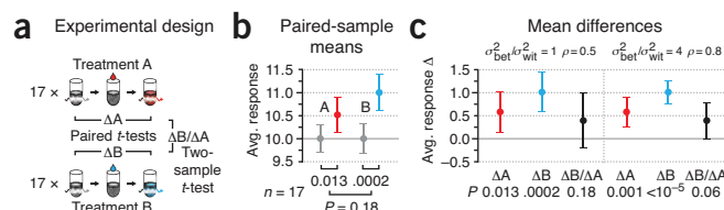
Figure 3 | Design and reporting for a paired, single-factor experiment. (a) The same n = 17 sample is used to measure the difference between treatment and background ( \Delta A = A_{\text{after}} - A_{\text{before}} , \Delta B = B_{\text{after}} - B_{\text{before}} ), analyzed with the paired t -test. Two-sample t -test is used to compare the difference between responses ( \Delta B versus \Delta A ). (b) Simulated sample means and P values for measurements and comparisons in a. (c) Mean difference, CIs and P values for two variance scenarios, \sigma_{\text{bet}}^2 / \sigma_{\text{wit}}^2 of 1 and 4, corresponding to \rho of 0.5 and 0.8. Total variance was fixed: \sigma_{\text{bet}}^2 + \sigma_{\text{wit}}^2 = 1 . All error bars show 95% CI.
