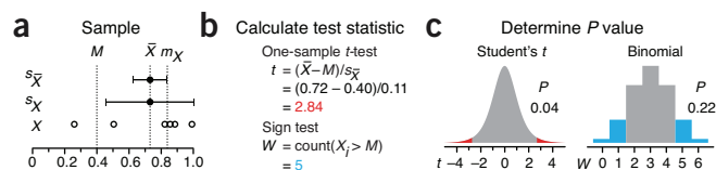
Figure 1 | A sample can be easily tested against a reference value using the sign test without any assumptions about the population distribution.
