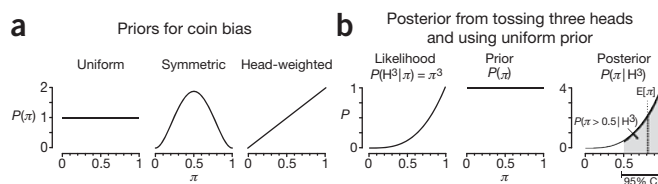
Figure 1 | Prior probability distributions represent knowledge about the coin before it is tossed. (a) Three different prior distributions of \pi , the probability of heads. (b) Toss outcomes are combined with the prior to create the posterior distribution used to make inferences about the coin. The likelihood is the probability of observing a given toss outcome, which is \pi^3 for a toss of H^3 . The gray area corresponds to the probability that the coin is biased toward heads. The error bar is the 95% credible interval (CI) for \pi . The dotted line is the posterior mean, E(\pi) . The posterior is shown normalized to 4\pi^3 to make its area 1.
