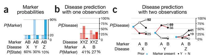
Figure 3 | Disease predictions based on presence of markers.
