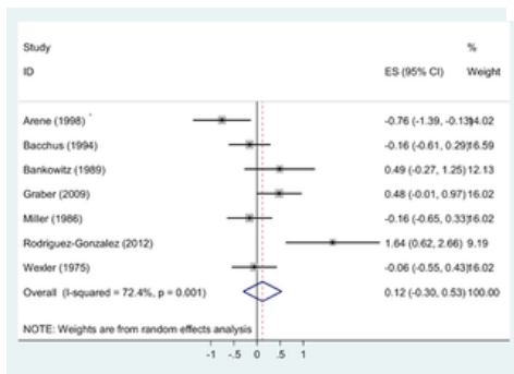
Fig 8. Two-groups meta-analysis: Forest plot of the accurate diagnosis retrieval rates of DDX generators compared to other types of clinical diagnoses.
