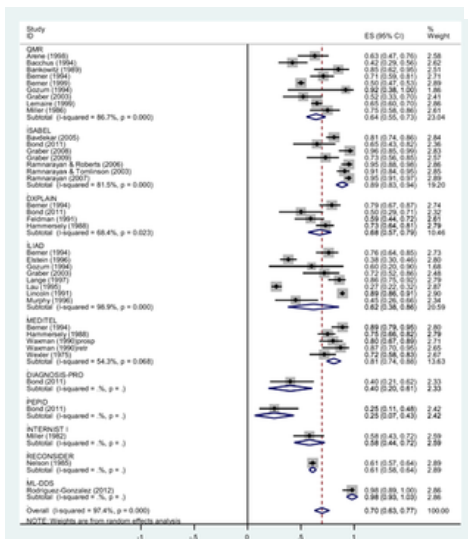
Fig 4. Single-group meta-analysis: Forest plot of the accurate diagnosis retrieval rates by subgroups of DDX generators.
