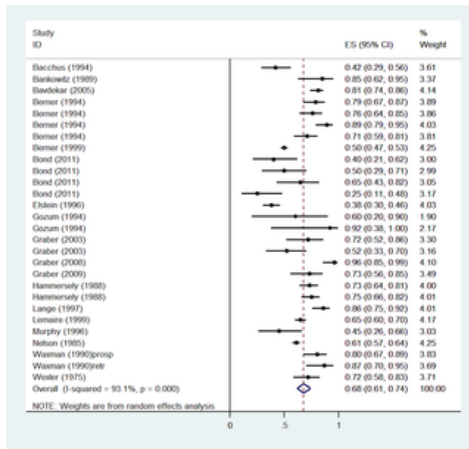
Fig 5. Sensitivity analysis: Forest plot of the rates of accurate diagnosis retrieval of DDX generators across studies with stronger methodological quality ratings.
