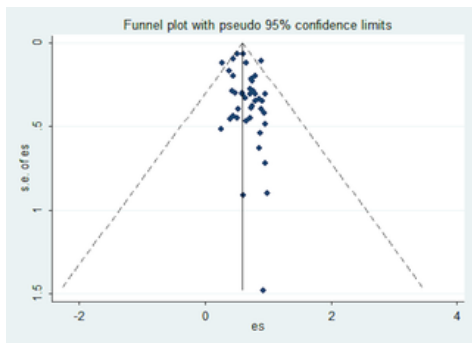
Fig 7. Funnel plot for studies examining the accurate diagnosis retrieval rates of DDX generators.
