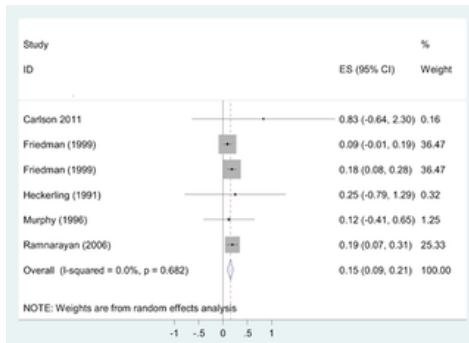
Fig 9. Two-groups meta-analysis: Forest plot of the accurate diagnosis retrieval rates of DDX generators in before-after studies.
