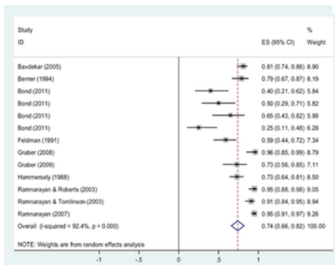
Fig 6. Sensitivity analysis: Forest plot of the rates of accurate diagnosis retrieval of DDX generators across studies testing commercially available DDX generators.
