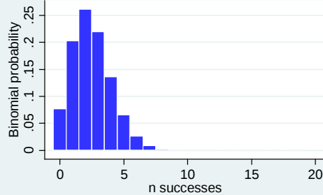
n=50 p=0.05
