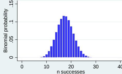
n=50 p=0.35
