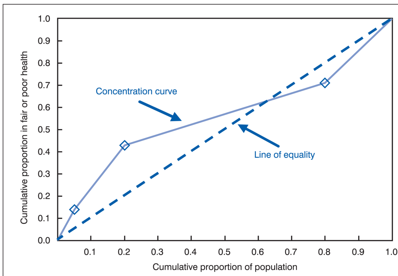
Figure 6. Concentration curve for hypothetical population 2
