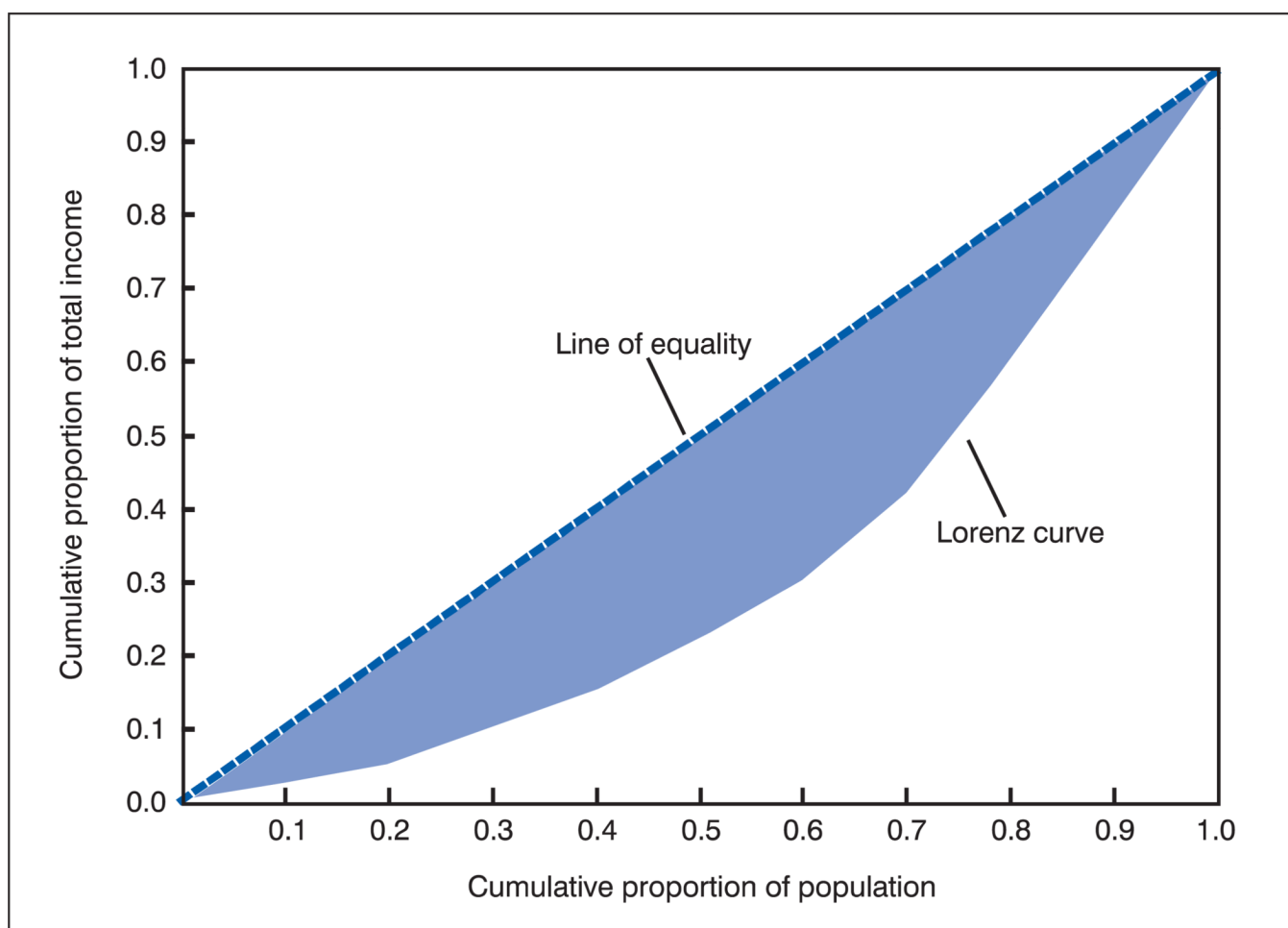
Figure 4. Lorenz curve for a hypothetical population
