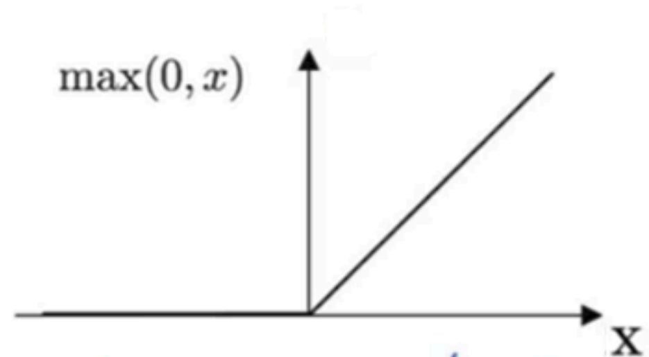
ReLU Function
