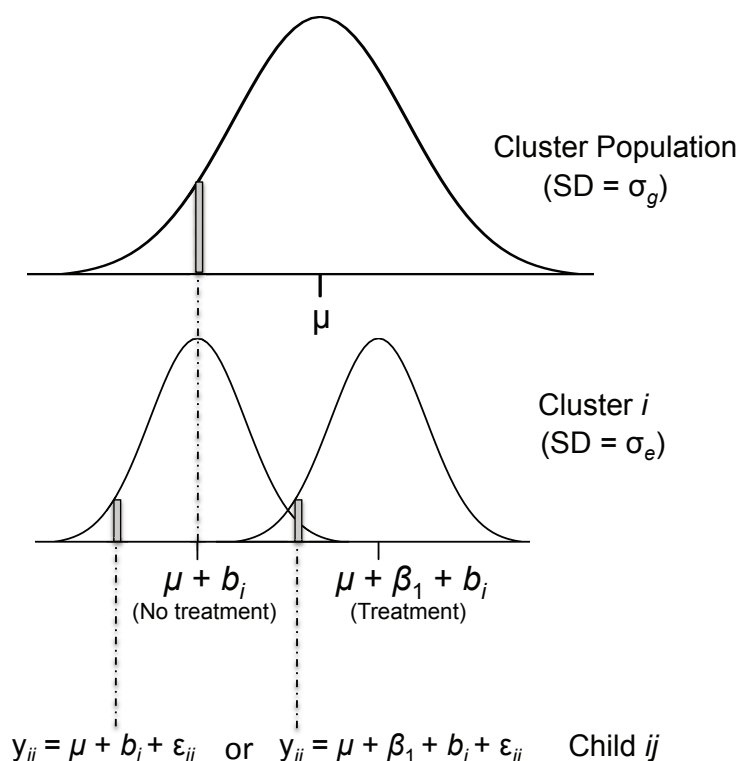
Figure 2 Summary of random effects draws used in a basic simulation of a cluster-level intervention with individual-level outcomes ( y_{ij} ). The population mean is \mu , b_i are random effects at the cluster level and \varepsilon_{ij} are random errors at the individual level. \beta_1 is the assumed difference in y_{ij} for individuals in treated clusters versus individuals in control clusters.
