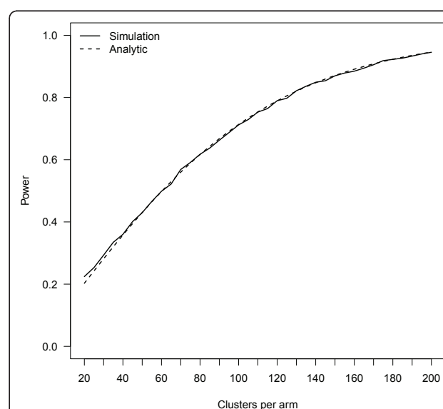
Figure 4 Power curves (1-Type II error) using the simulation approach versus a conventional analytic formula for a simple cluster-randomized design described in the text.
