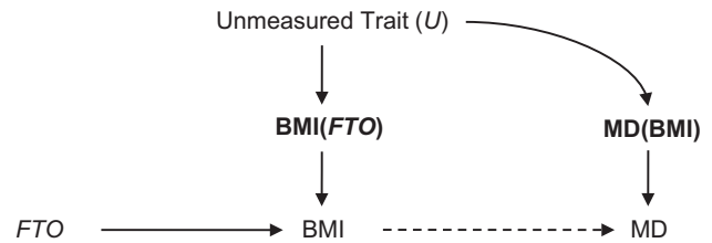
Figure 3. Directed acyclic graph showing that positive confounding arises from the association between counterfactuals. BMI( FTO ) represents the set of counterfactual values of body mass index (BMI) for all possible values of fat mass and obesity-associated ( FTO ) genotype. MD(BMI) represents the set of counterfactual values of mental disorder (MD) for all possible values of BMI. An unmeasured trait ( U ) does not affect FTO , but U does affect the value BMI would take for any specific value of FTO .
