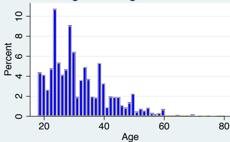
Histogram of age with 50 bins
