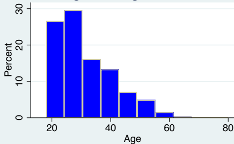
Histogram of age with 10 bins
