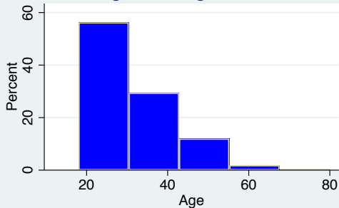
Histogram of age with 5 bins
