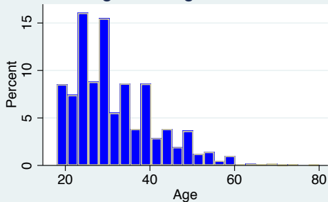
Histogram of age with 25 bins
